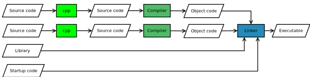
Figure 16.1: Compilation
