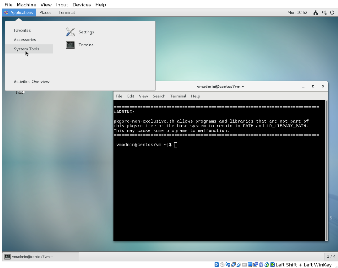
Figure 41.2: CentOS 7 with Gnome Desktop as a Guest under VirtualBox
