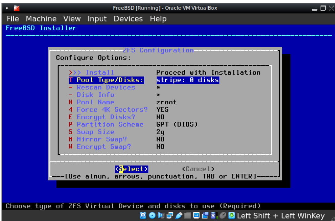
Figure 37.2: FreeBSD Installer ZFS Options
