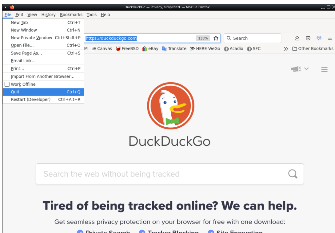
Figure 3.1: Hot Keys
