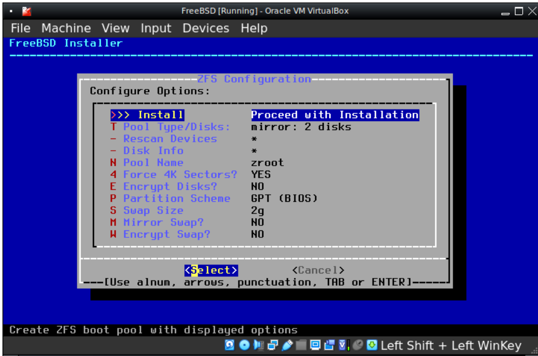
Figure 37.5: FreeBSD Installer ZFS Commit
