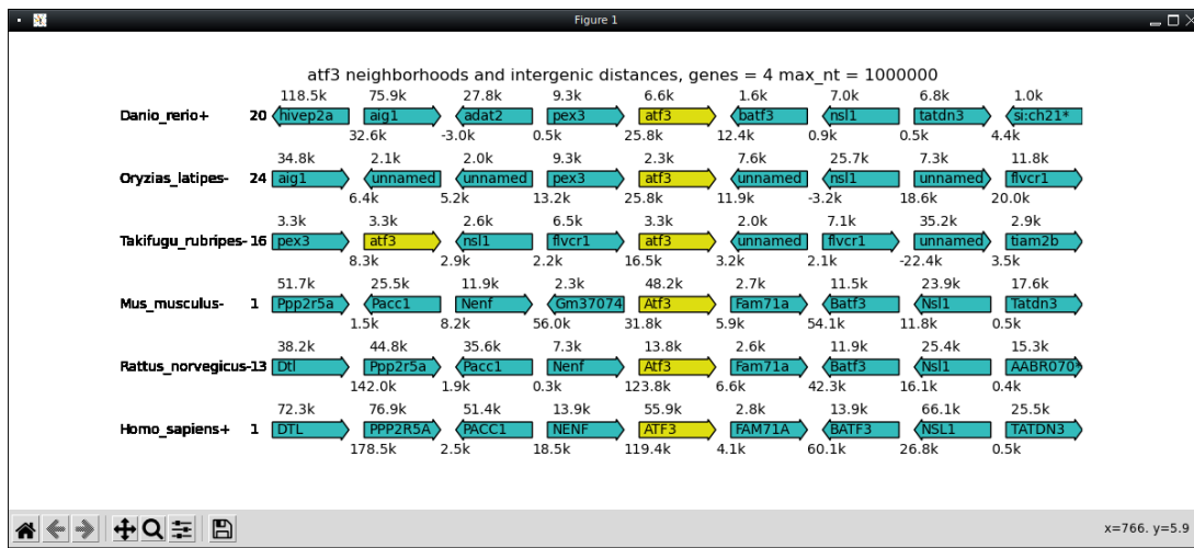
Figure 2.2: Visualizing Gene Neighborhoods with Matplotlib
