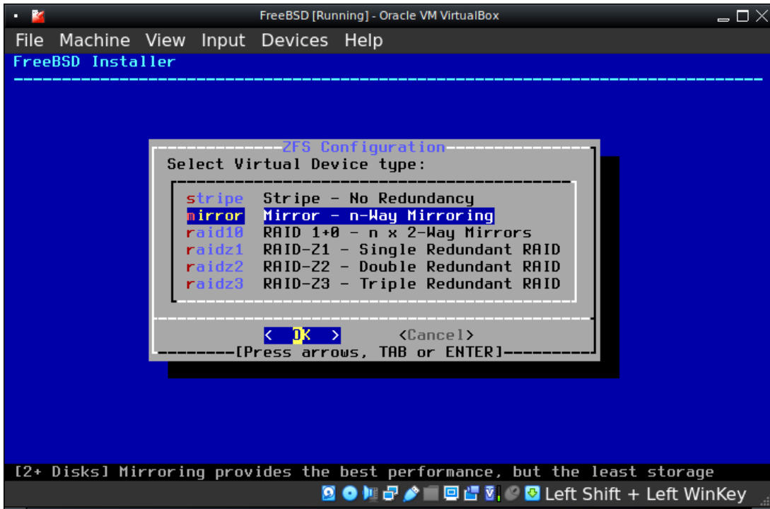
Figure 37.3: FreeBSD Installer ZFS RAID Level Selection
