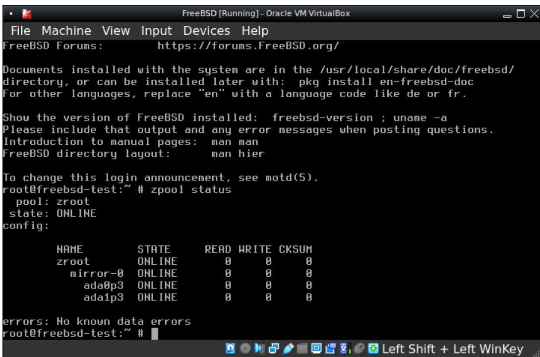
Figure 37.6: FreeBSD ZFS Status
